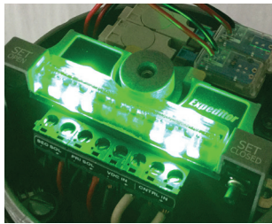
Open position
