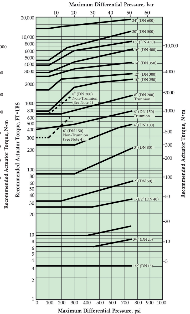
Xtreme (X) and TFM (Z) Seated Valves 1/2" - 12" (DN 15 - 300)
