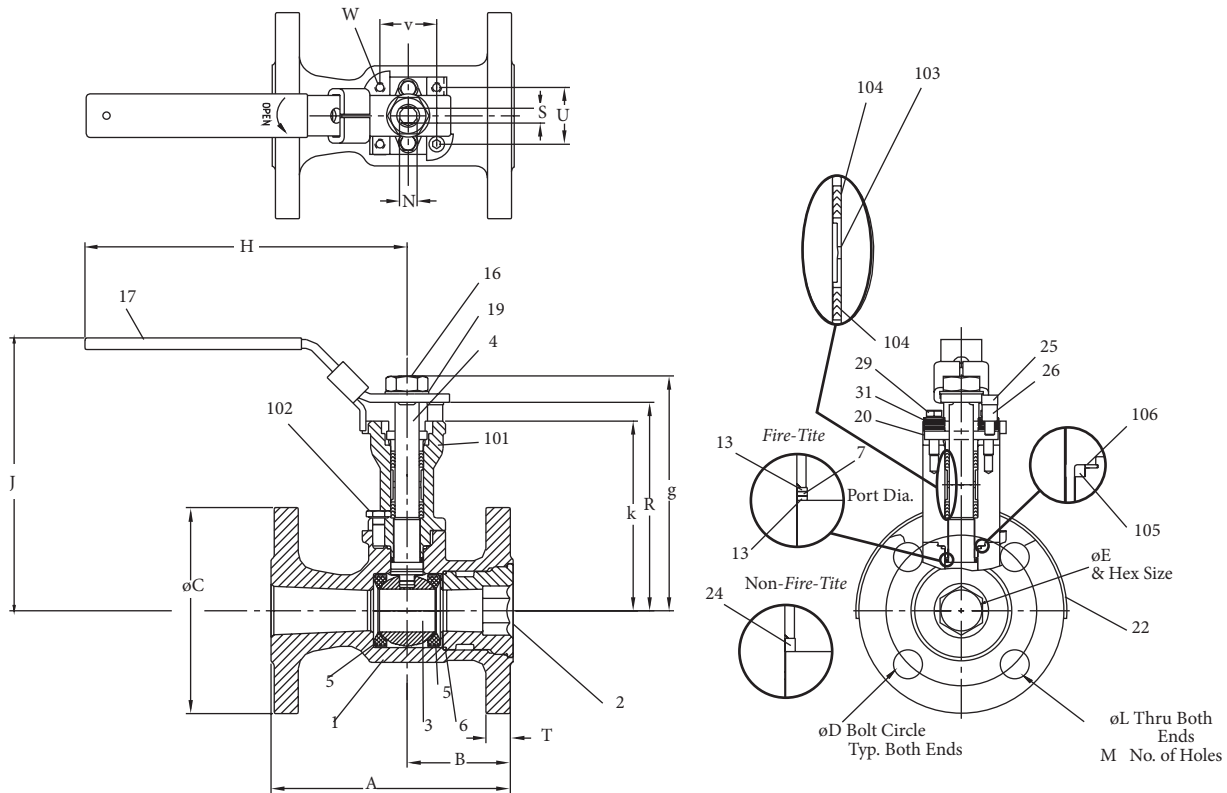
1/2" - 1-1/2" (DN15 - 40) Series 9150 ASME Class 150 and Series 9300 ASME Class 300 with Emission-Pak (Non-Trunnion)
