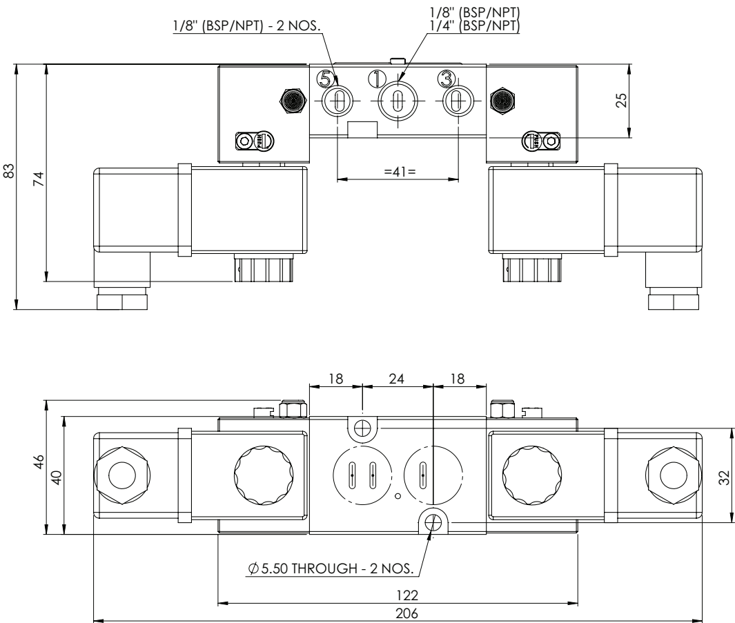
VAQNC114/ 214 SERIES
