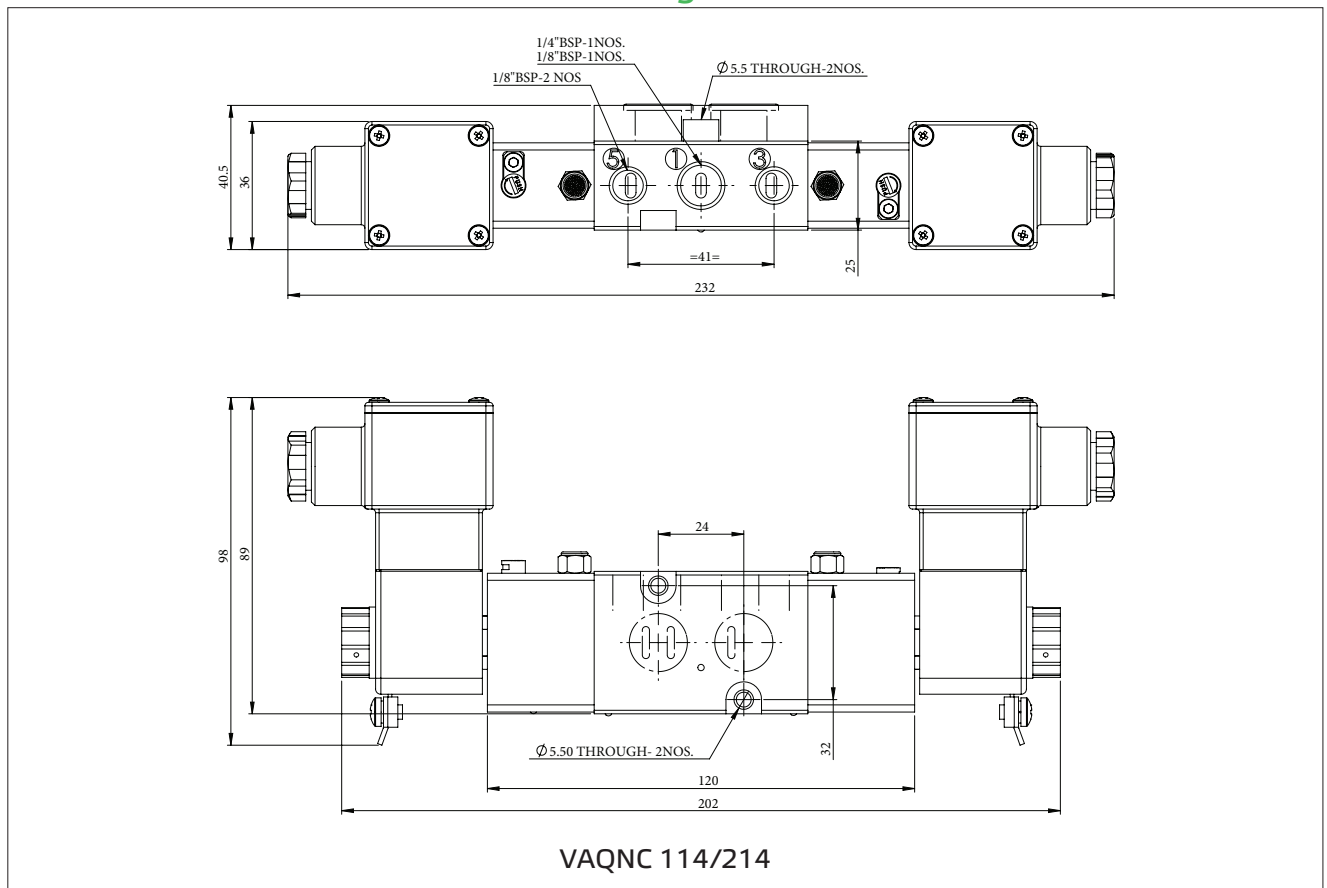
Figure 6 VAQNC114/214
