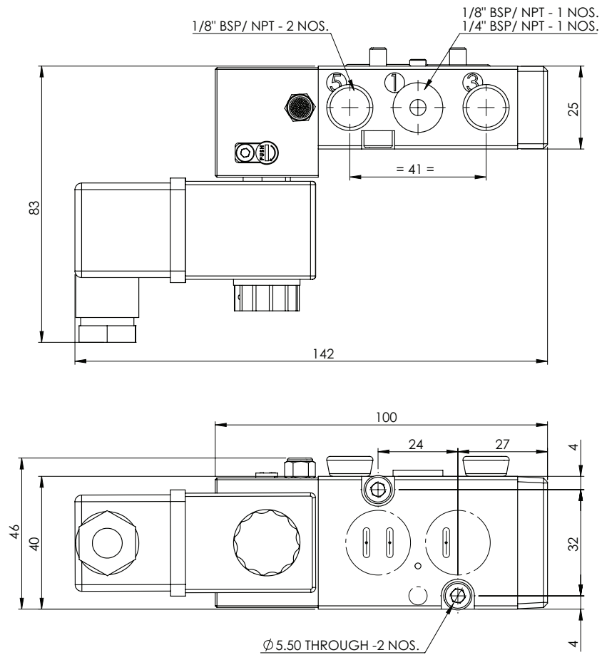
VAQNC 113/213 SERIES
