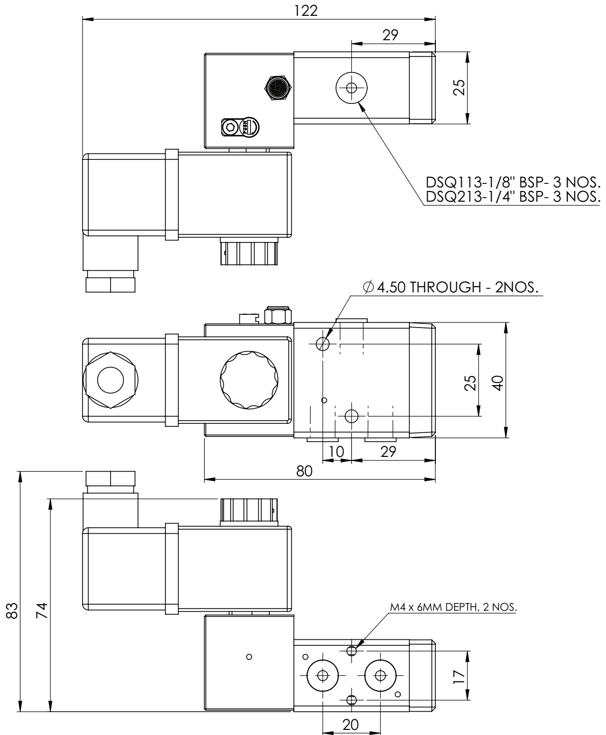
DSQ 113/213 Series With Exia Nass Magnet Coil
